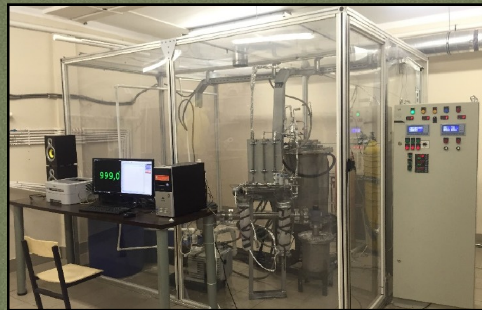
Pyrolytic Boron Nitride Deposition Plant 1.0
